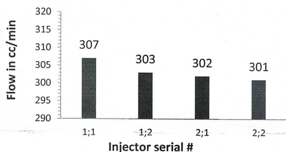
Injector Flow before Cleaning
